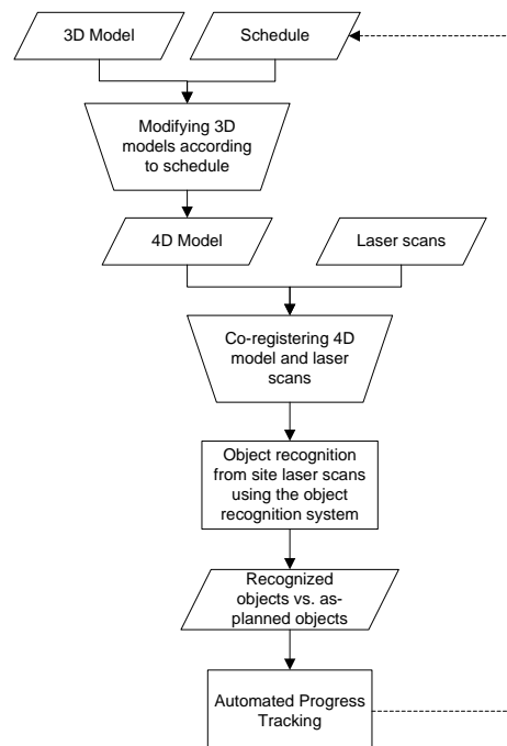
Figure 2 Conceptual view of the components of the proposed approach
