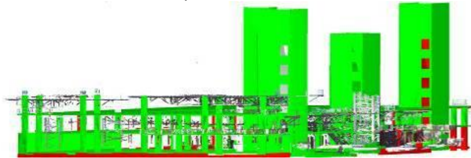
Figure 9 Non matched cloud points and the 4D model colored based on the recognition results (red: planned but not recognized; green: planned and recognized). Note that the elements colored in red at the bottom of the building are foundation elements that were already covered at the time of the scan.
