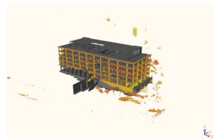
Figure 6 3D model referenced in the scanner's spherical coordinate frame.
